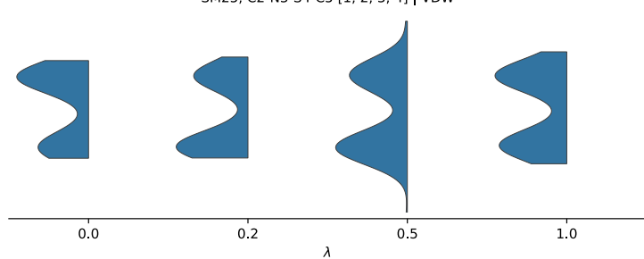
SM25, C2-N3-S4-C5 [1, 2, 3, 4] | VDW
