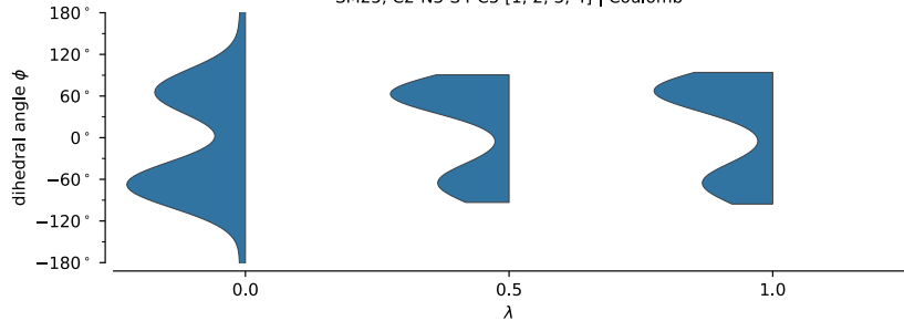
SM25, C2-N3-S4-C5 [1, 2, 3, 4] | Coulomb
