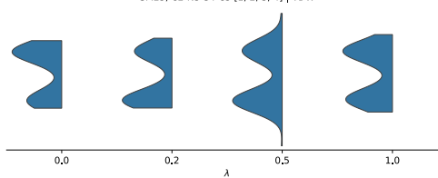
SM25, C2-N3-S4-C5 [1, 2, 3, 4] | VDW
