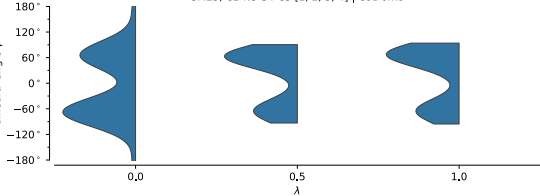
SM25, C2-N3-S4-C5 [1, 2, 3, 4] | Coulomb
