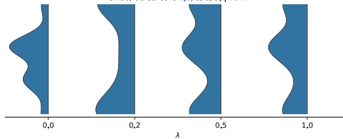
SM26, O1-S2-C3-C4 [0, 1, 2, 3] | VDW
