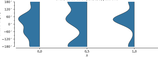
SM26, O1-S2-C3-C4 [0, 1, 2, 3] | Coulomb
