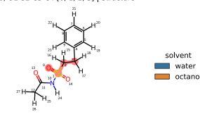
SM26, O1-S2-C3-C4 [0, 1, 2, 3] | Structure
