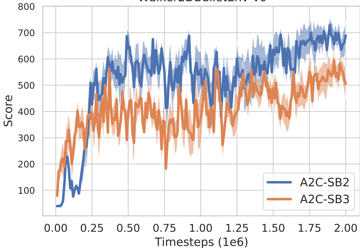
Walker2DBulletEnv-v0
