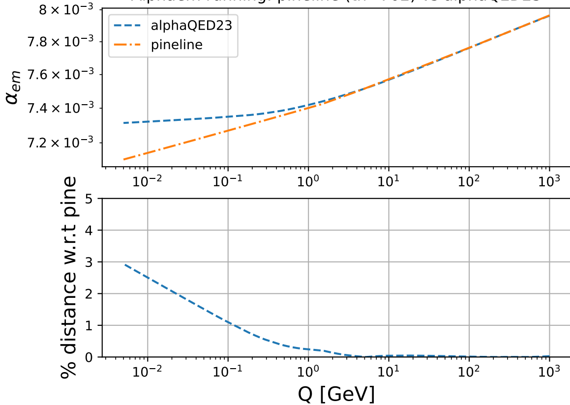
Alphaem running: pipeline (th=702) vs alphaQED23
