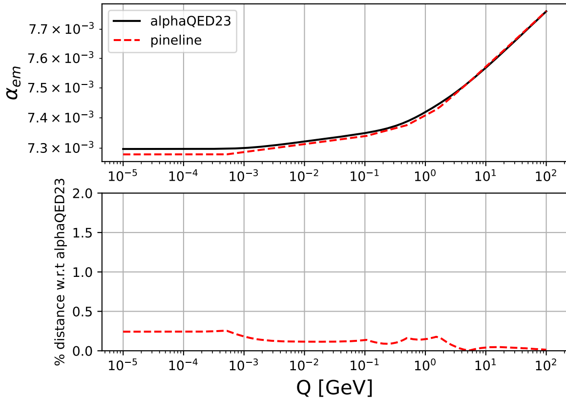
Alphaem running: pipeline (th=702) vs alphaQED23, m_q=0.5 GeV
