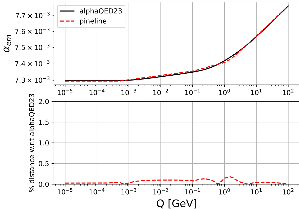
Alphaem running: pineline (th=702) vs alphaQED23, m_q=1 GeV
