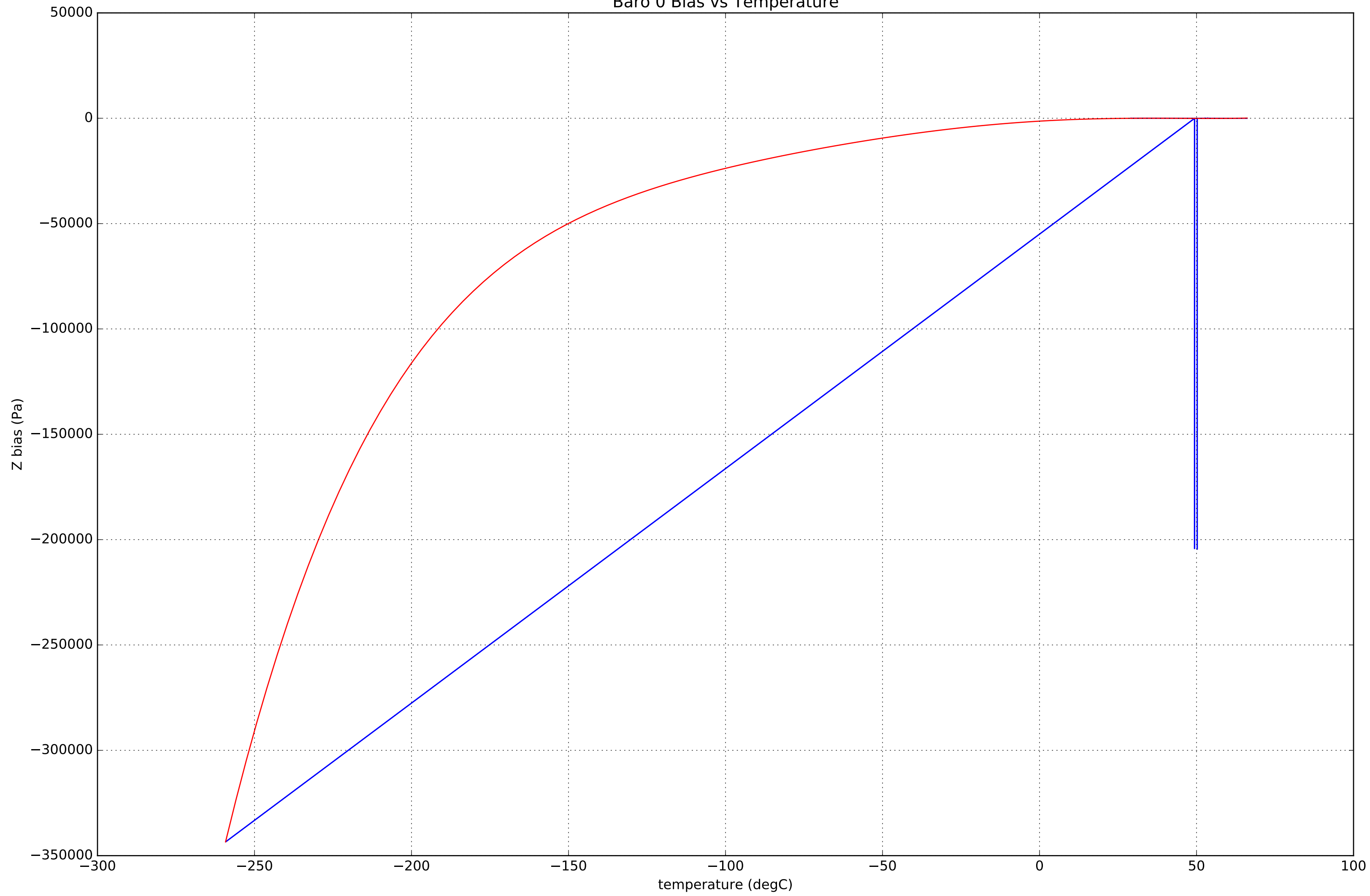
Baro 0 Bias vs Temperature
