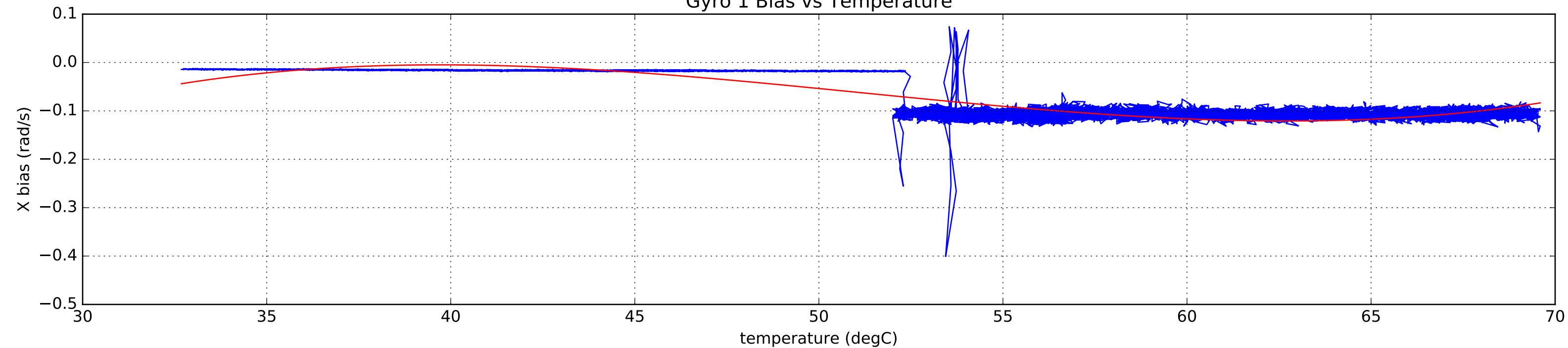
Gyro 1 Bias vs Temperature
