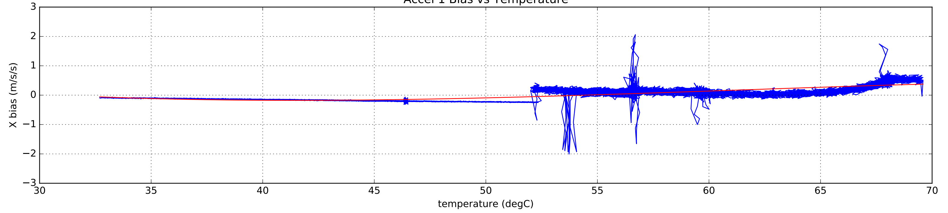
Accel 1 Bias vs Temperature
