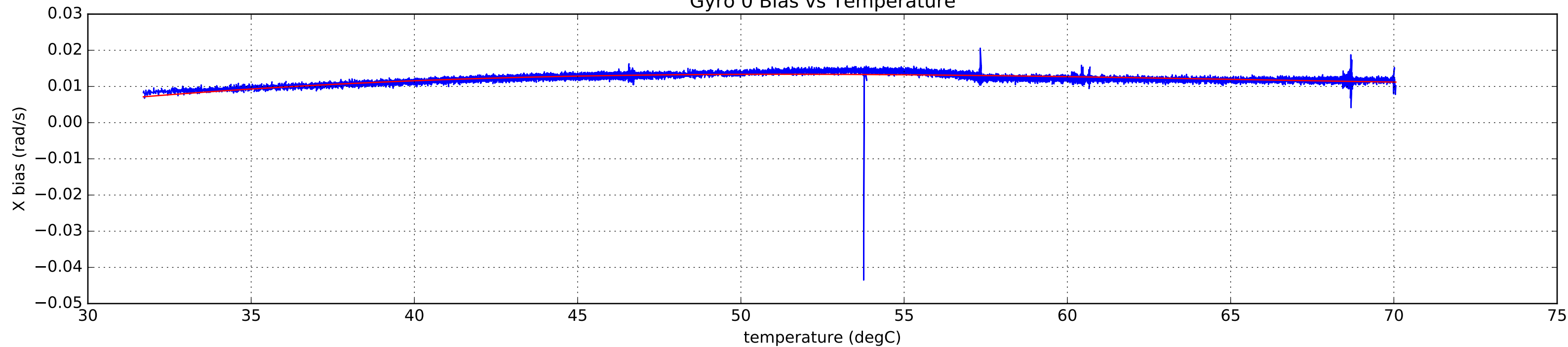
Gyro 0 Bias vs Temperature
