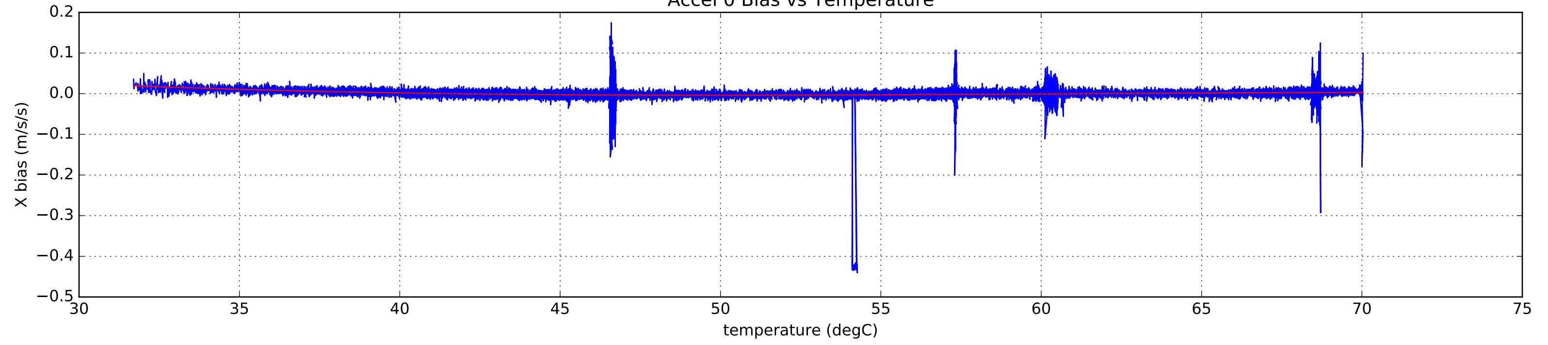
Accel 0 Bias vs Temperature
