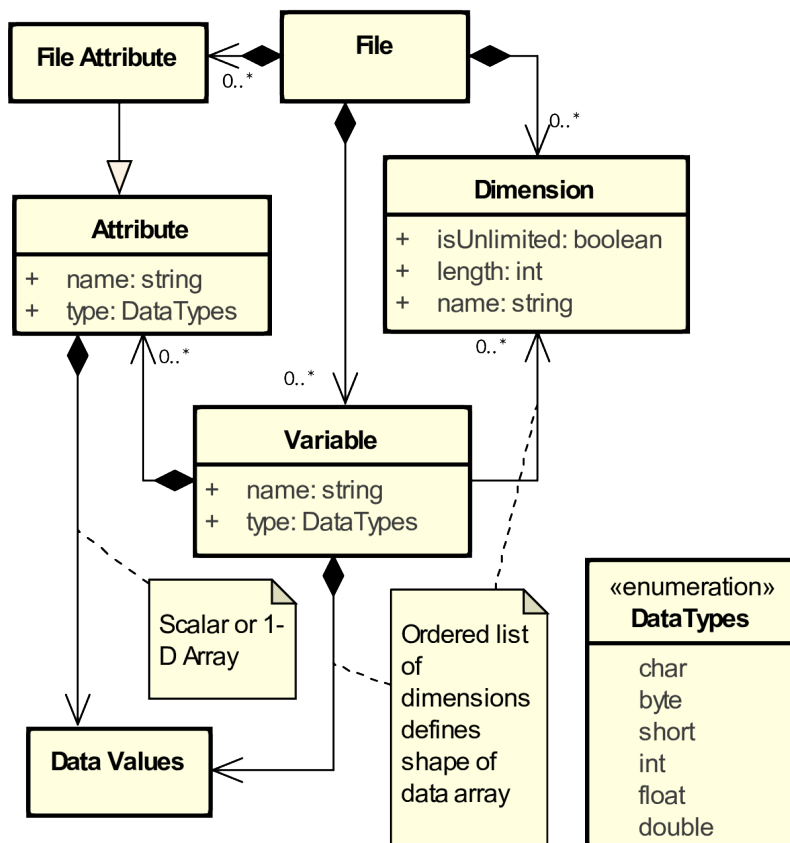
Figure 7. Key components of the netCDF classic data model. Files consist of global attributes, dimensions and variables. Variables contain attributes and data, and attributes also contain data. Variables, attributes and dimensions all contain properties, such as a "name" which identifies them in the file. A data array has a data type for all of its elements (e.g. "double" for 64-bit floating point numbers).
