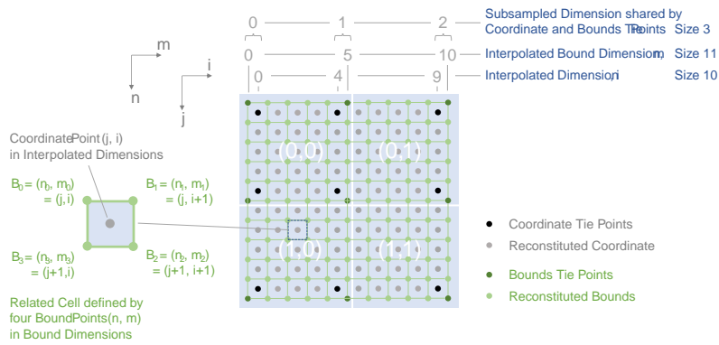
Figure 6. Example of 2D bounds interpolation showing the bounds tie points and reconstituted bound points within a continuous area consisting of four interpolation subareas. The dimensions are shown for one of the two axes only. The index relationship between coordinate point indices and the related bound points indices is indicated.
