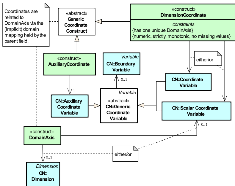
Figure 10. The relationship between domain axis, dimension coordinate and auxiliary coordinate constructs and CF-netCDF (defined in figure 2 and identified here with the "CN" prefix). A dimension or auxiliary coordinate construct is defined by a CF-netCDF coordinate, scalar coordinate or auxiliary coordinate variable, and the associated CF-netCDF boundary variable if it exists. A generic coordinate construct spans one or more domain axis constructs, but the mapping of which ones is only held by the parent field construct.
