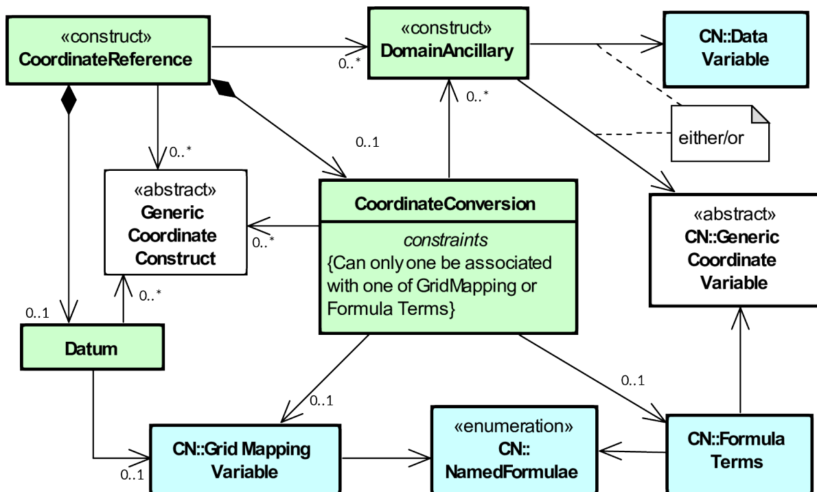
Figure 11. The relationship between coordinate reference and domain ancillary constructs and CF-netCDF (defined in figure 2 and identified here with the "CN" prefix). A coordinate reference construct is defined either by a grid mapping variable, or a formula_terms attribute of a CF-netCDF coordinate variable. The coordinate reference construct is composed of generic coordinate constructs, a datum, and a coordinate conversion formula. The coordinate conversion formula is usually defined by a named formula in the CF conventions. A domain ancillary construct term of a coordinate conversion formula is defined by a CF-netCDF data variable or a CF-netCDF generic coordinate variable.
