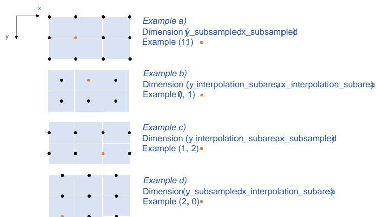
Figure 5. Through combination of dimensions, interpolation parameter variables may provide values for a) interpolation subareas sharing a tie point, b) each interpolation subarea, c) and d) interpolation subareas sharing a boundary.
