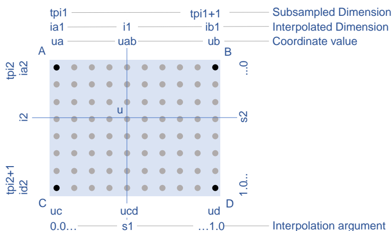
Figure 13. Two-dimensional interpolation subarea.
