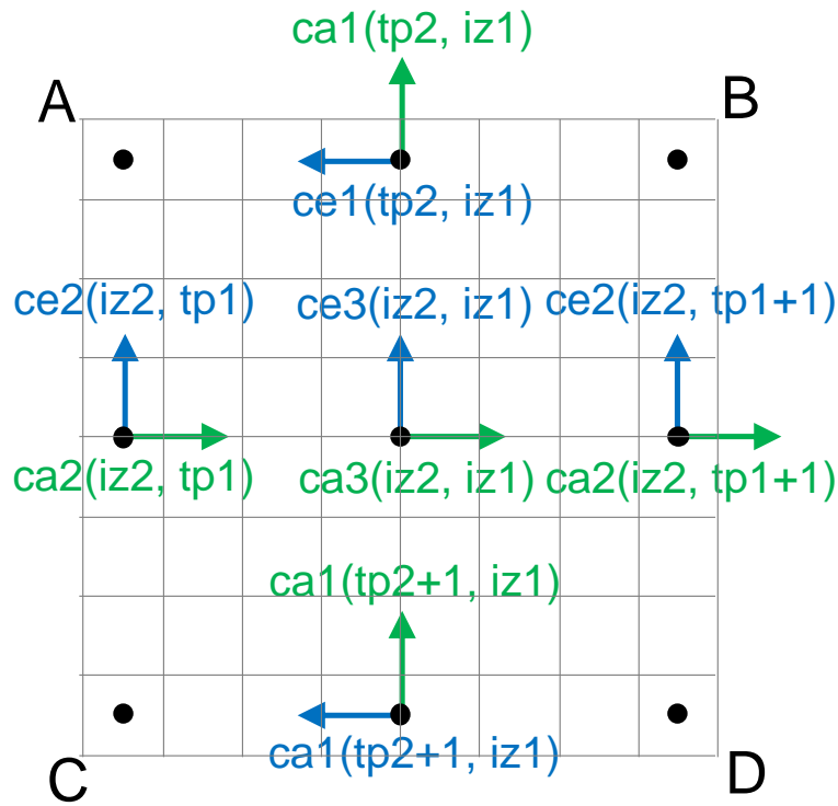
Figure 16. The parametric representation of the interpolation coefficients cea = (ce, ca) , stored in the interpolation parameters ce1 , ca1 , ce2 , ca2 , ce3 and ca3 , is equivalent to five additional tie points for the interpolation subarea. Shown with parameter orientation and indices.
