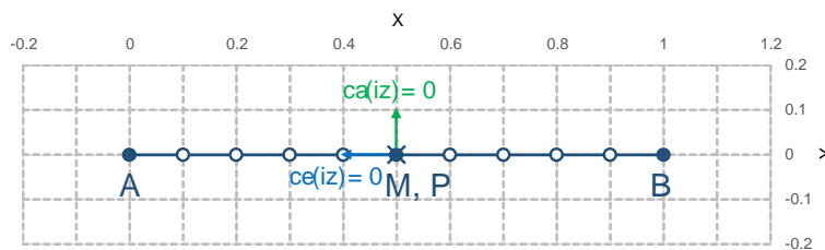
Figure 14. With the expansion coefficient ce = 0 and the alignment coefficient ca = 0 , the method reconstitutes the points at regular intervals along a great circle between tie points A and B .
