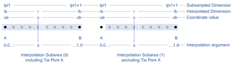
Figure 12. One-dimensional interpolation subareas, one including and one excluding tie point A.
