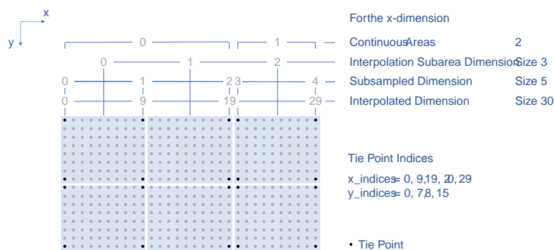
Figure 4. Overview of the different dimensions for coordinate interpolation.
