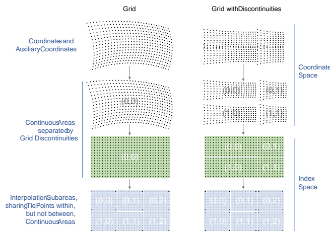
Figure 3. Process for generating the interpolation subareas for a grid without discontinuities and for a grid with discontinuities.
