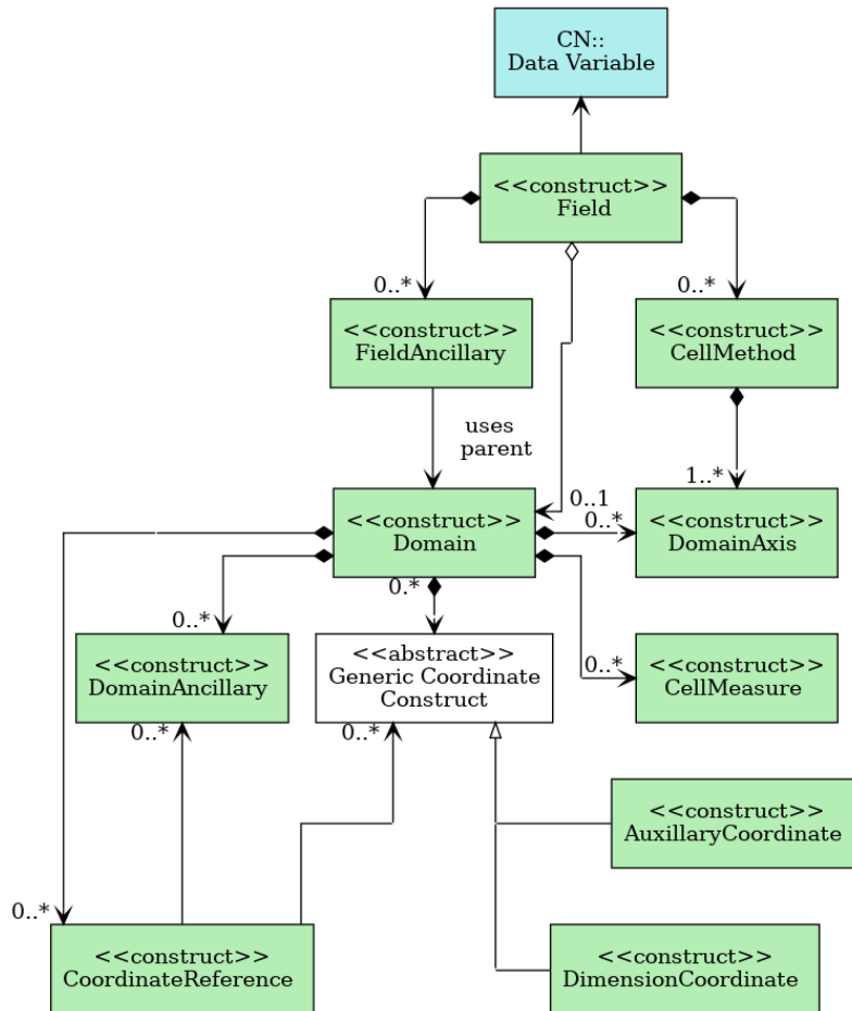
Figure 9. The constructs of the CF data model. The field construct corresponds to a CF-netCDF data variable (defined in figure 2 and identified here with the "CN" prefix). Relationships between other constructs and CF-netCDF are given in figure 4 and figure 5. The domain construct provides the linkage between the field construct and the constructs which describe measurement locations and cell properties. It is useful to define an abstract generic coordinate construct that can be used to refer to coordinates when their type (dimension or auxiliary coordinate construct) is not an issue.
