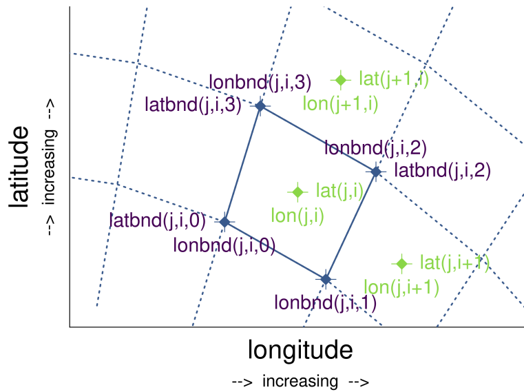
Figure 2. Order of \text{lonbnd}(j, i, 0) to \text{lonbnd}(j, i, 3) and of \text{latbnd}(j, i, 0) and \text{latbnd}(j, i, 3) in the case of two-dimensional horizontal coordinate axes. Tuples (\text{lon}(j, i), \text{lat}(j, i)) represent grid cell centers and tuples (\text{lonbnd}(j, i, n), \text{latbnd}(j, i, n)) represent the grid cell vertices.
