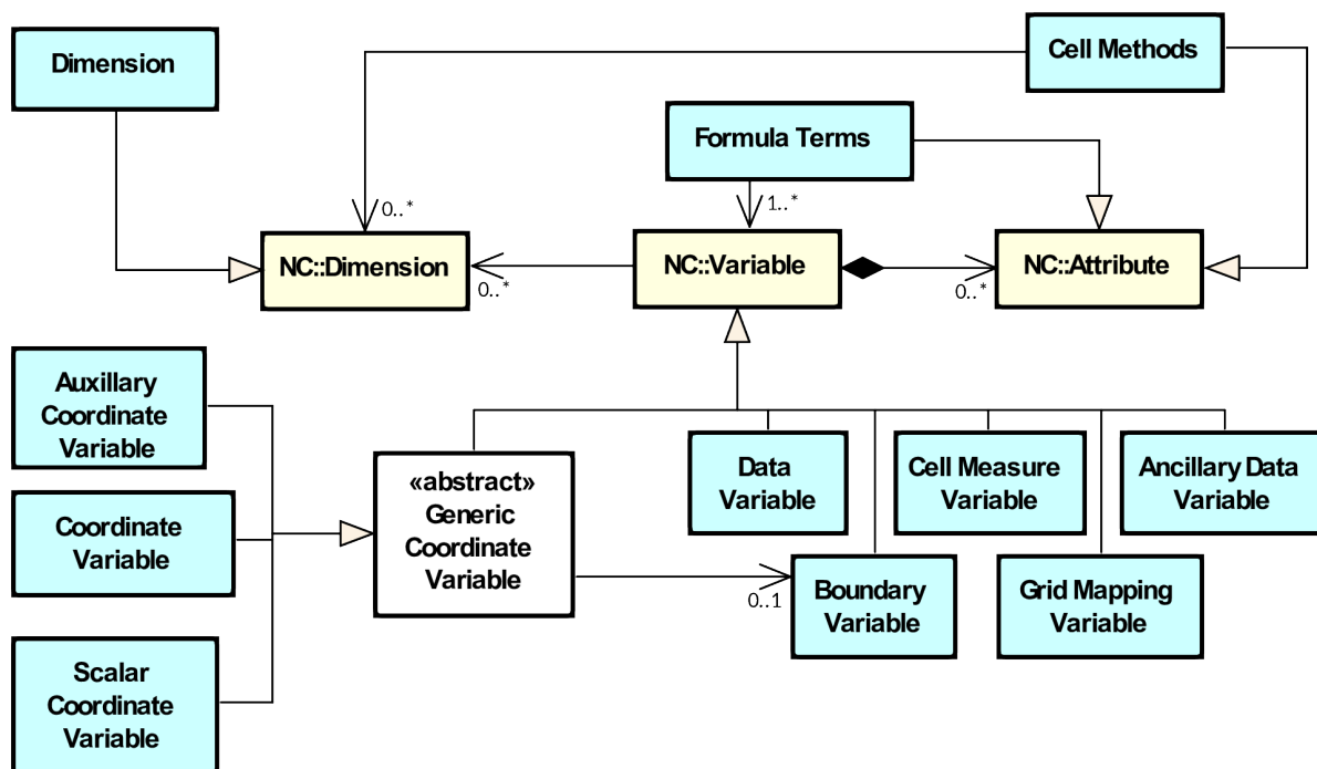
Figure 8. The relationships between CF-netCDF elements and their corresponding netCDF variables, dimensions and attributes (defined in figure 3 and identified here with the "NC" prefix). It is useful to define an abstract generic coordinate variable that can be used to refer to coordinates when their type (coordinate, auxiliary or scalar coordinate variable) is not an issue. The CF convention details the mechanisms which are used in the netCDF file to express the relationships among the CF-netCDF elements, but these are not shown.
