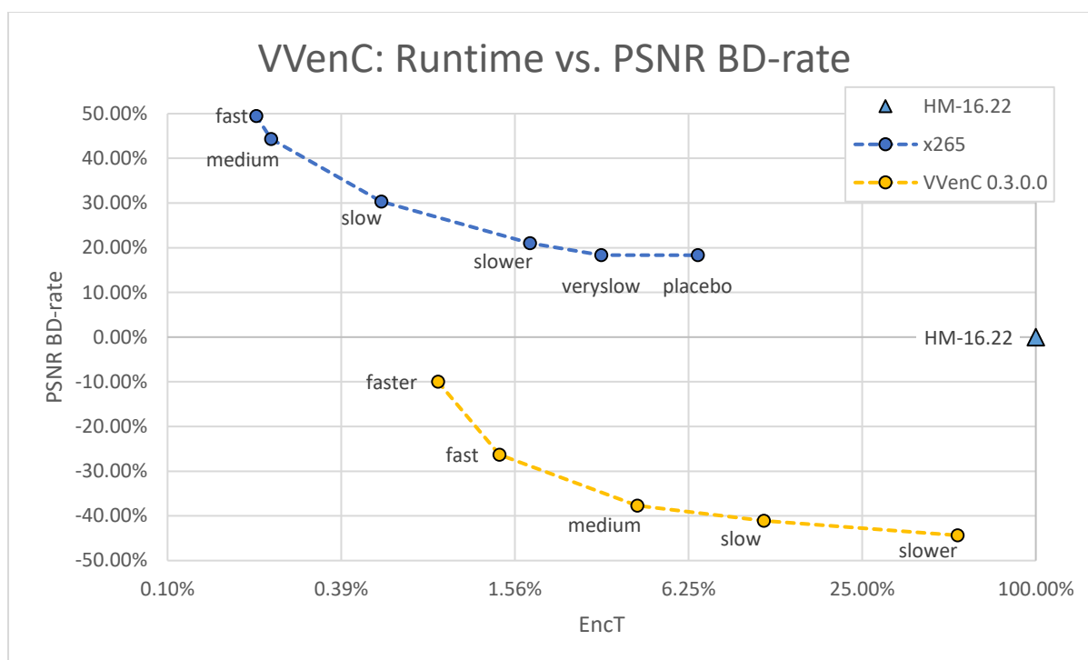
Figure 2: PSNR BD-rate gain and relative encoder runtime in comparison to HM-16.22 for VVenC and x265 running with 8 threads. Lower PSNR BD-rate values mean a better compression for the same objective quality in terms of PSNR.
