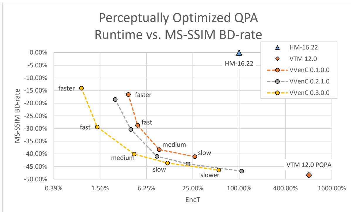
Figure 3: MS-SSIM BD-rate gain and encoder runtime in comparison to HM-16.22 for VTM and VVenC with perceptually optimized quantization parameter adaption enabled. VVenC results are given for the 5 preset options: faster, fast, medium, slow and slower. Lower MS-SSIM BD-rate values mean a better compression for the same quality in terms of MS-SSIM.
