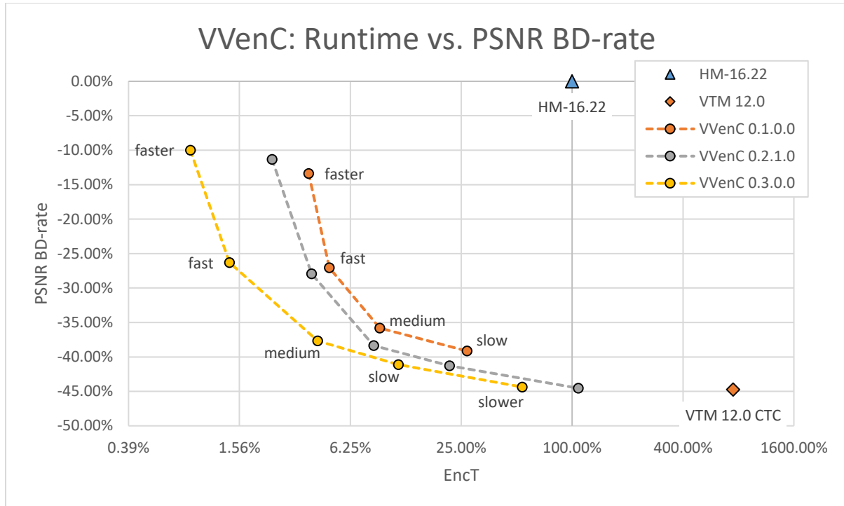
Figure 1: PSNR BD-rate gain and relative encoder runtime in comparison to HM-16.22 for VVenC and VTM. Results are given for the 5 preset options: faster, fast, medium, slow and slower. Lower PSNR BD-rate values mean a better compression for the same objective quality in terms of PSNR.
