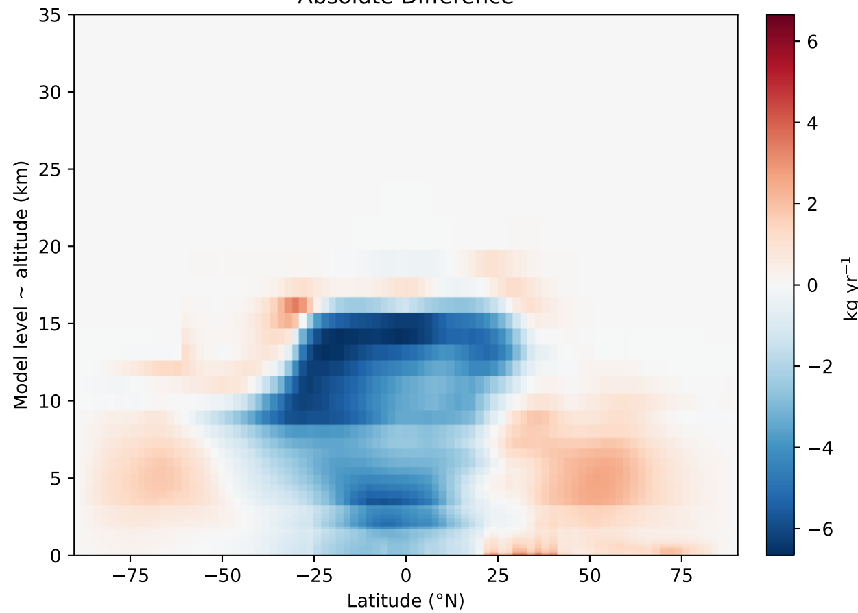
Absolute Difference
