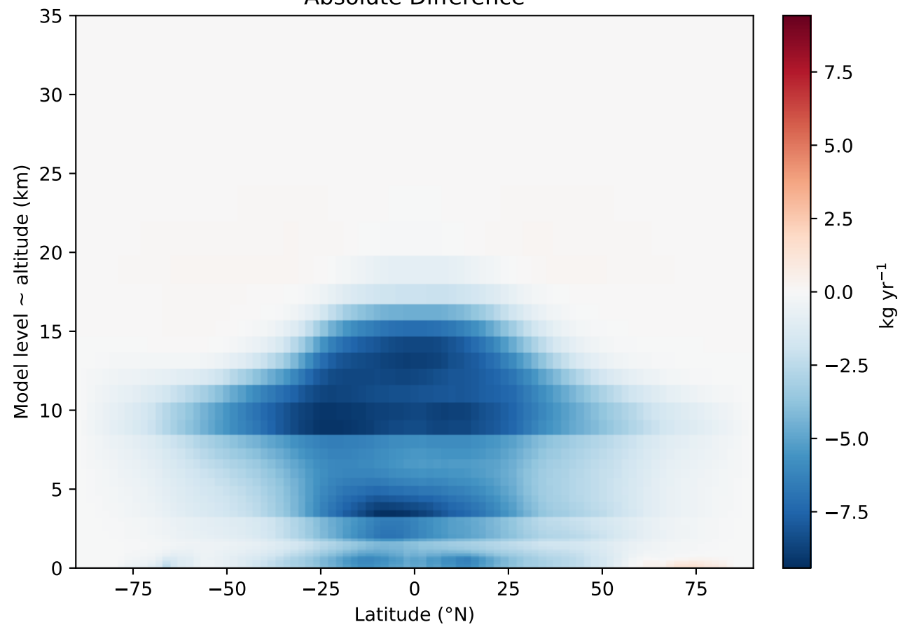
Absolute Difference
