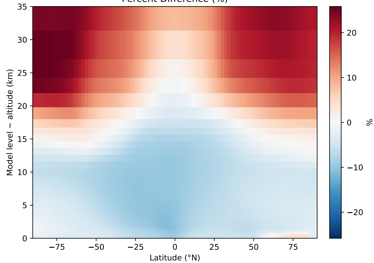
Percent Difference (%)
