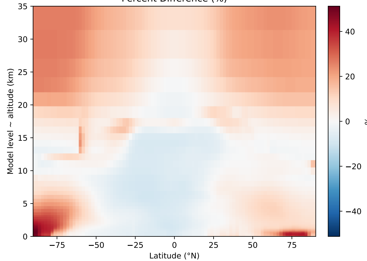
Percent Difference (%)
