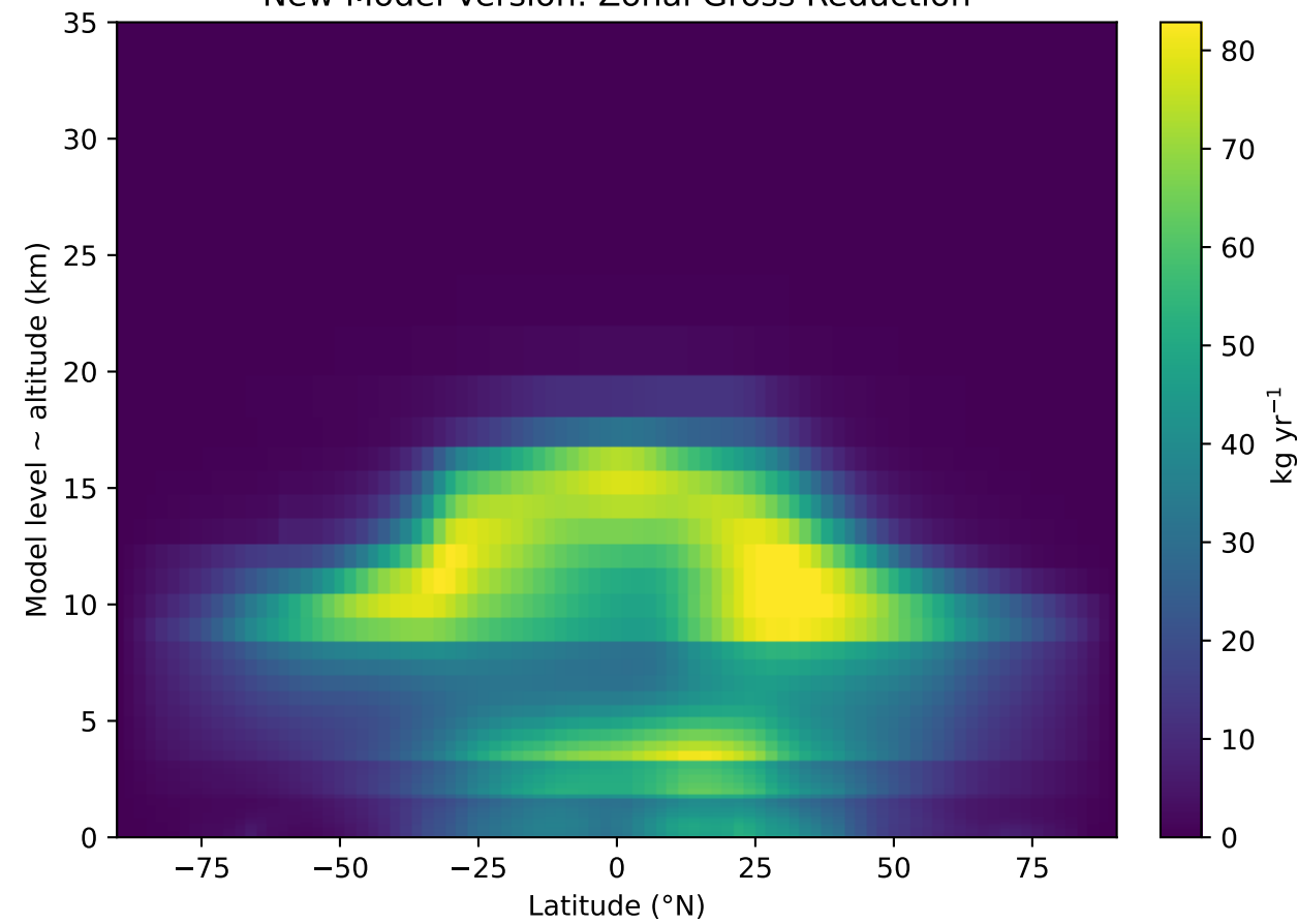
New Model Version: Zonal Gross Reduction
