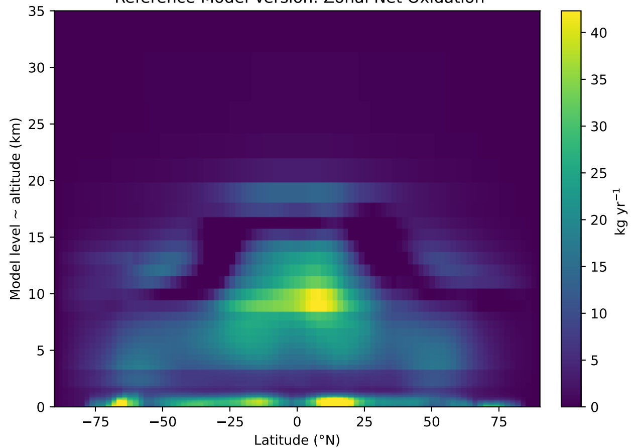
Reference Model Version: Zonal Net Oxidation
