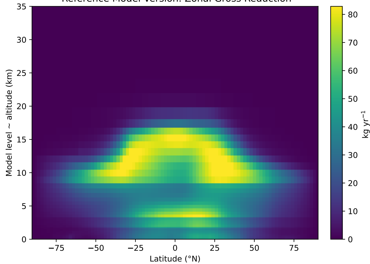
Reference Model Version: Zonal Gross Reduction
