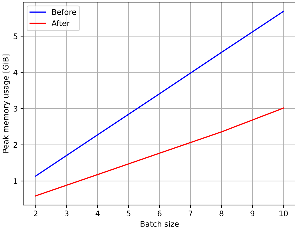
Meta-Llama-3-8B Input size 300, New tokens 2000
