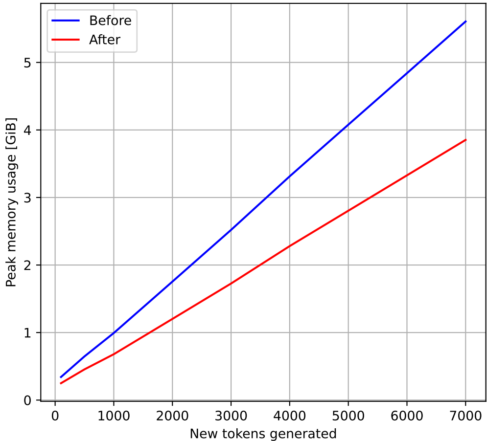
beam search Input size 300, Batch size 1 'num_beams': 2
