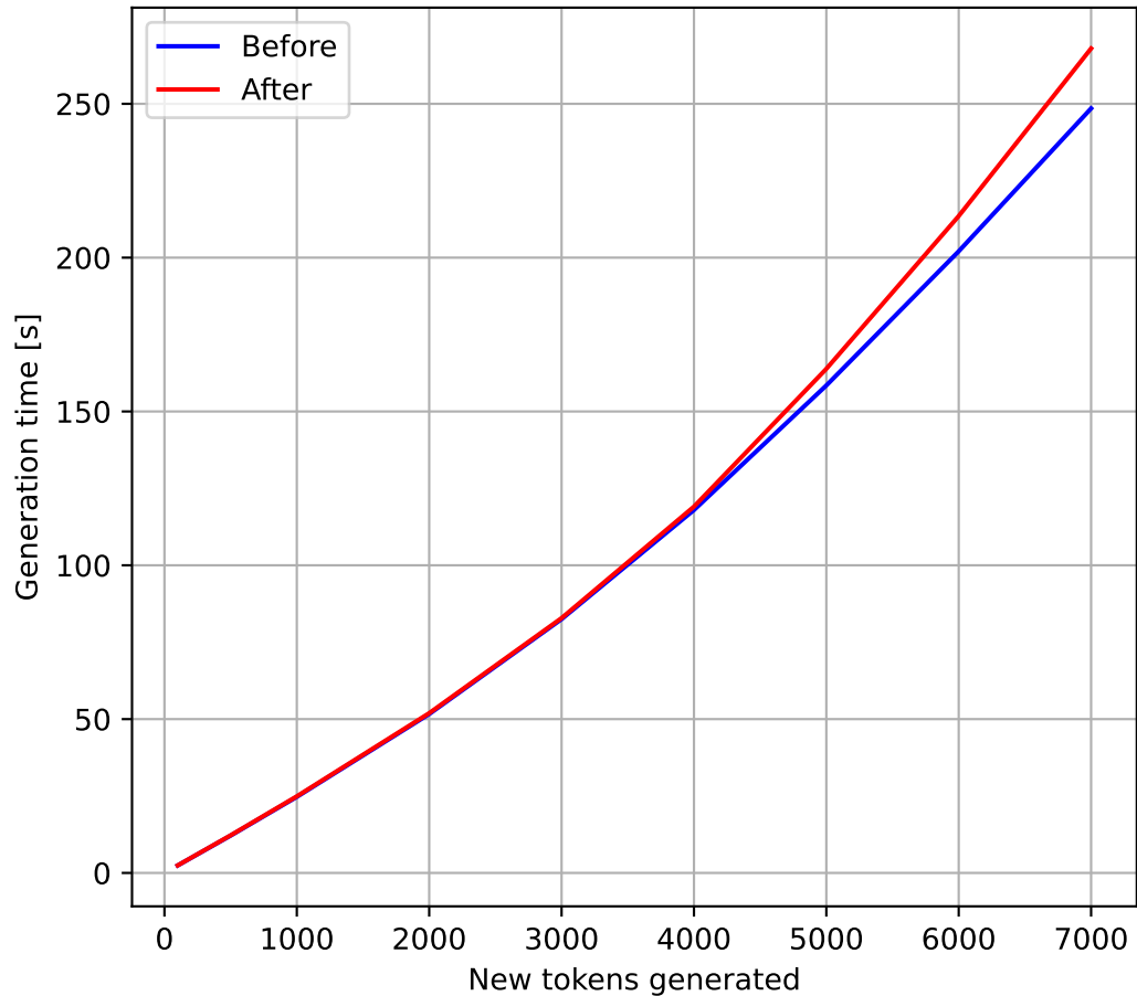
beam search Input size 300, Batch size 1 'num_beams': 2
