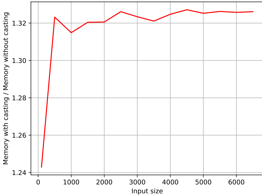
Mistral 7B
