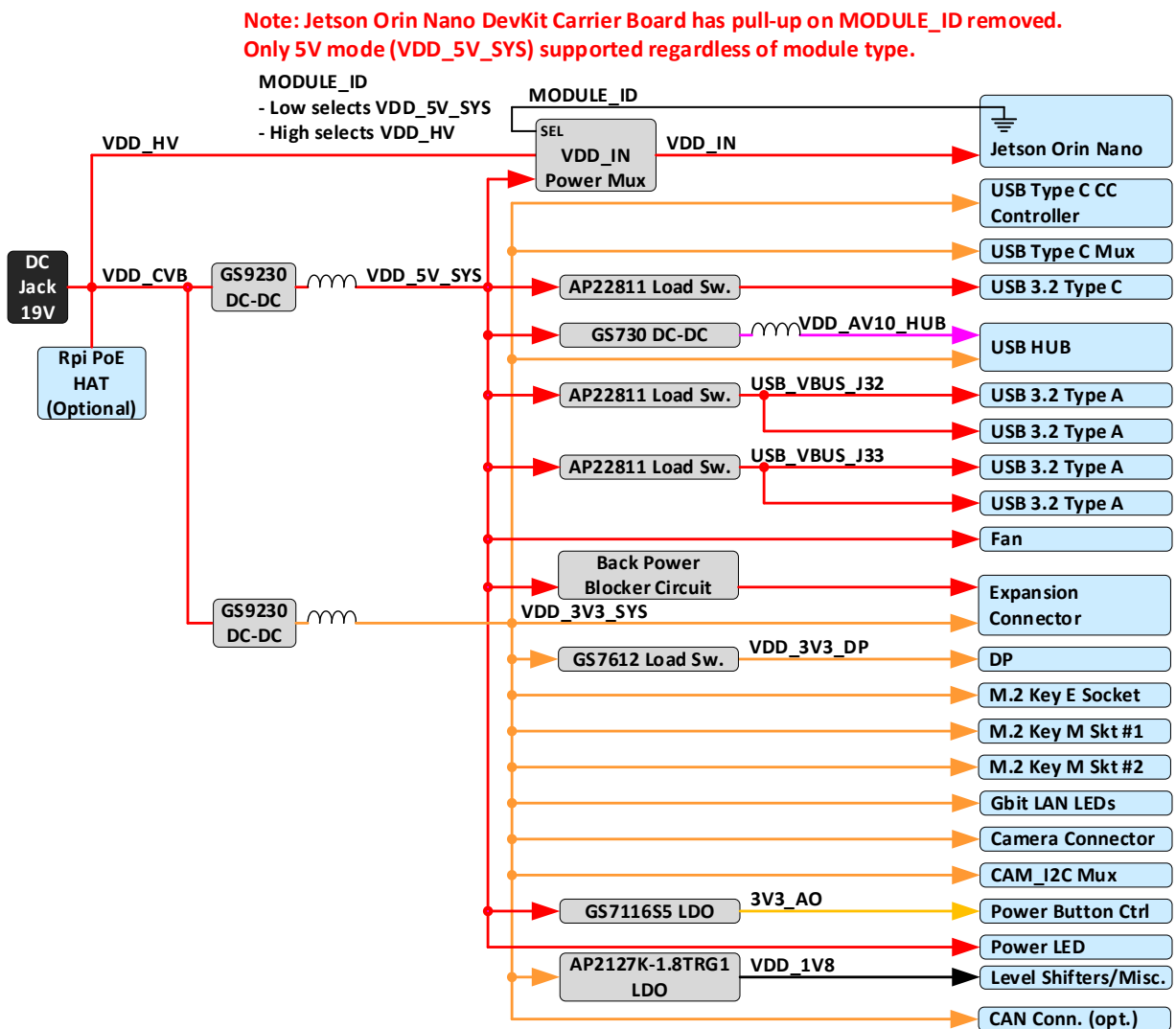
Figure 5-1. Power Diagram
