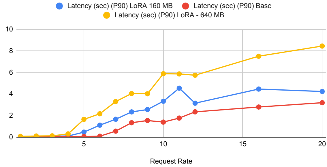
Latency (sec) (P90) LoRA 160 MB, Latency (sec) (P90) Base and Latency (sec) (P90) LoRA - 640 MB
