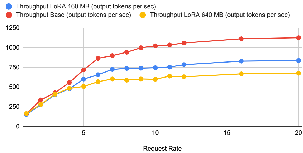
Throughput LoRA (output tokens per sec), Throughput Base (output tokens per sec) and Throughput LoRA 640 (output to...
